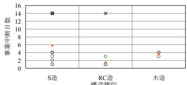
Fig.5. Relationship of structural type and recovery time in Table.2
