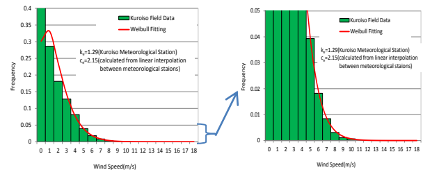
Figure3. Observed Wind Speed Frequency Distribution and Estimated Weibull Distribution at Kuroiso Field Test Site
