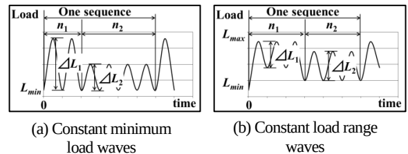
Figure 1. Repeating load waves used for fatigue test
