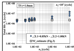
Figure 3. Variable amplitude load fatigue
