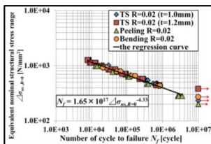
Figure 2. \Delta\sigma_{ns,R=0} - N_f
