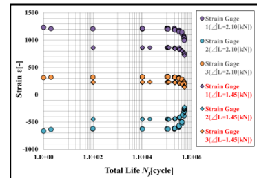
Figure 4. Measurement results of the strain displacement
