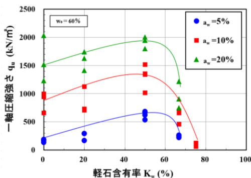
Fig. 2 Relationship between pumice content and unconfined compressive strength
