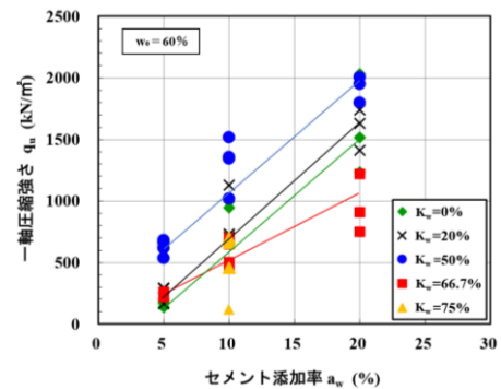
Fig. 3 Relationship between cement addition rate and unconfined compressive strength
