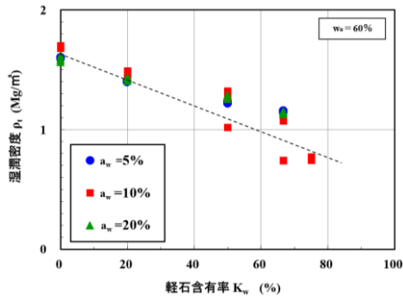
Fig. 1 Relationship between pumice content and wet density
