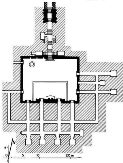
図2 Taung-Kyanzittha-umin の平面図 [2]
